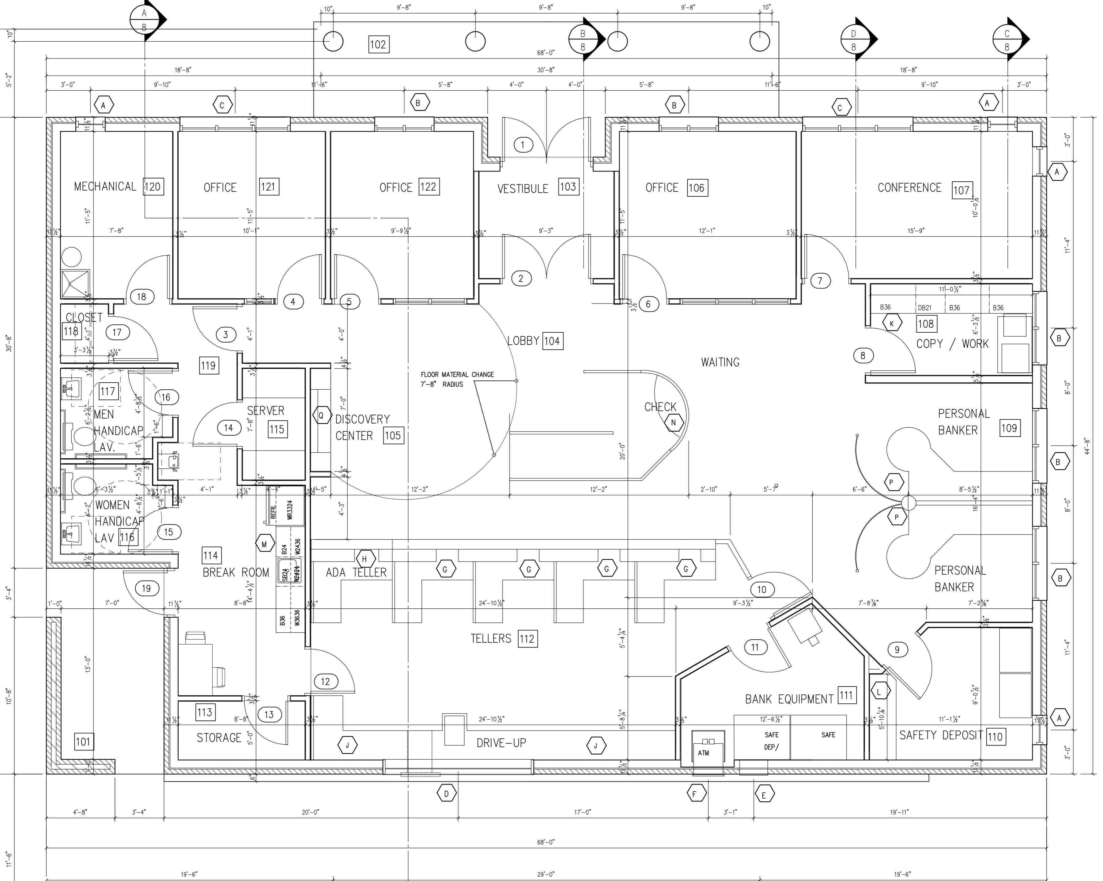
FLOOR PLAN SCALE - 1/4" = 1'-0" AREA = 2,904 SQ. FT.
