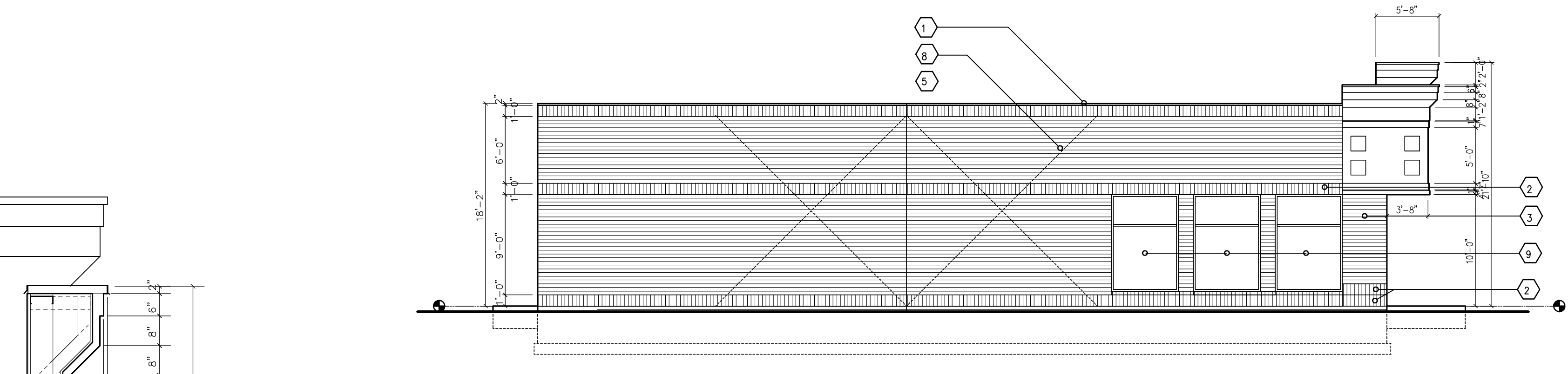
FRONT — NORTH ELEVATION
