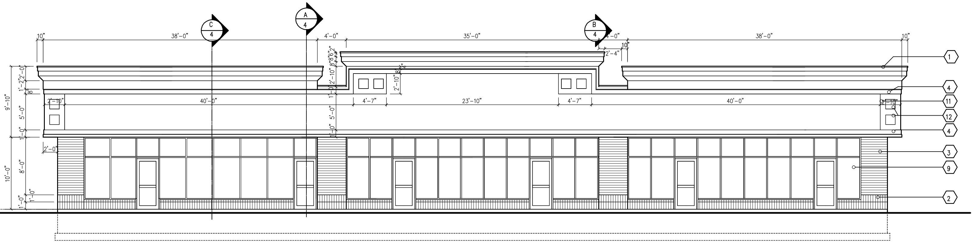
FRONT — NORTH ELEVATION
