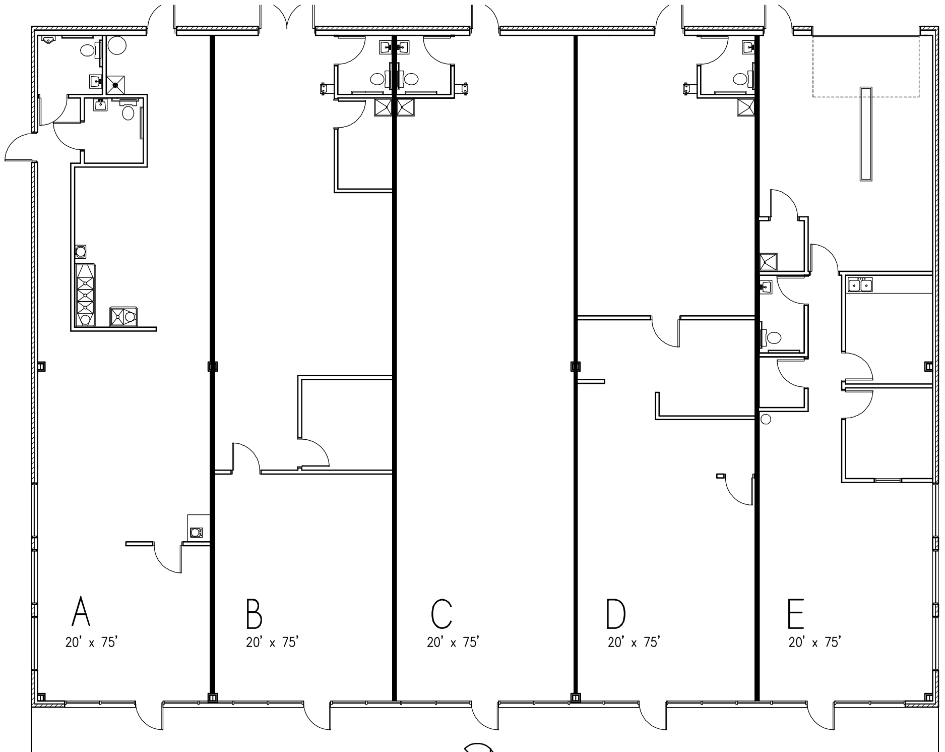
BUILDING FLOOR PLAN
